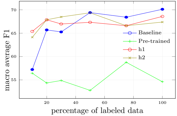
Figure 2: Performance on Founta et al. (2018) dataset.
