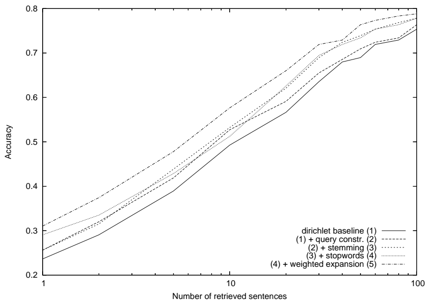
Figure 4: Number of retrieved sentences vs. accuracy for optimized smoothing methods
