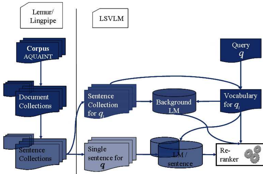
Figure 2: The sentence retrieval architecture for our experiments
