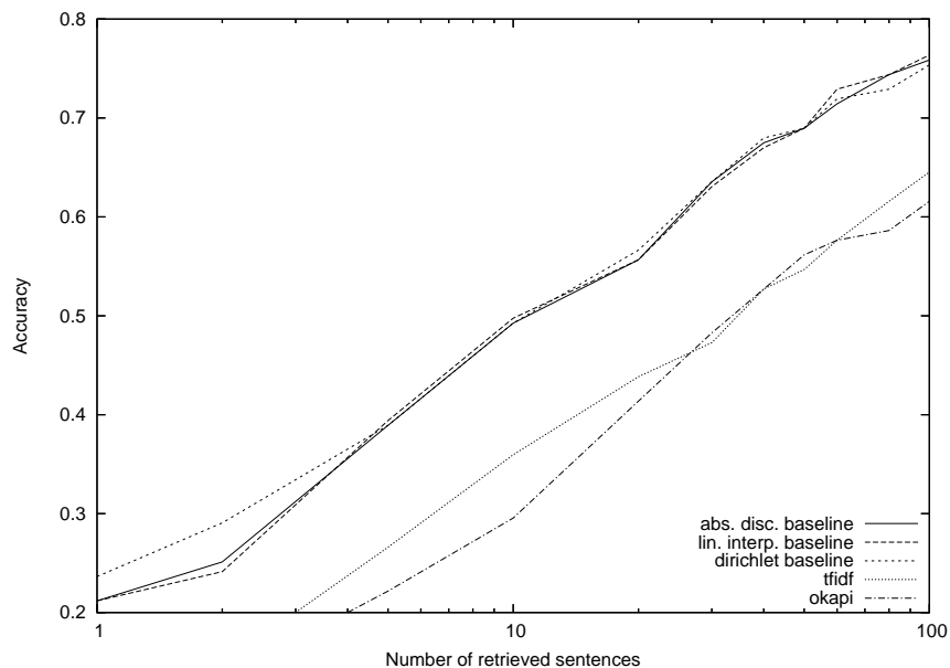
Figure 3: Number of retrieved sentences vs. accuracy for baseline experiments
