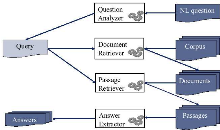
Figure 1: A general architecture for question answering systems
