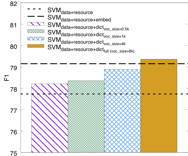
Figure 3: Comparison of SVM classifiers using dictionaries with different vocabulary sizes. dict full is equivalent to the SVM feature dict in Table 5.
