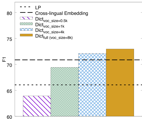
Figure 2: Comparison of dictionaries with different vocabulary sizes. Classifiers use no labeled training data . Dict full is equivalent to the dictionary shown in Table 5.
