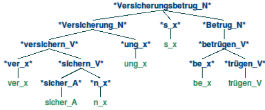
Figure 1: Morphological sample parse for Versicherungsbetrug ‘insurance fraud’
